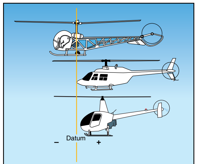
Figure 7-3. While the horizontal reference datum can be anywhere the manufacturer chooses, most small training helicopters have the horizontal reference datum 100 inches forward of the main rotor shaft centerline. This is to keep all the computed values positive.
