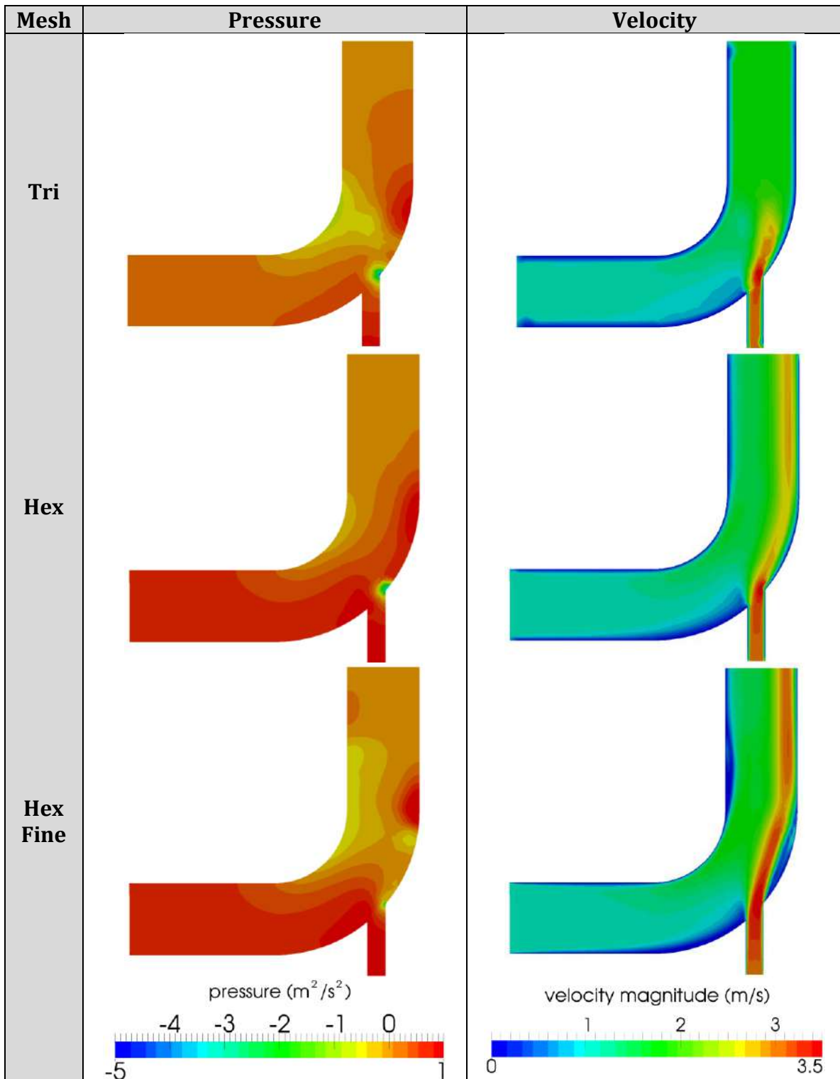
Figure 1.2 Comparison of different mesh type results at t = 75 s
